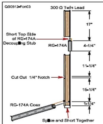
Figure 3 — The original DBJ-1 dual-band J-pole. The dimensions given assume that the antenna is inserted into a 3/4 inch Class 200 PVC pipe.
