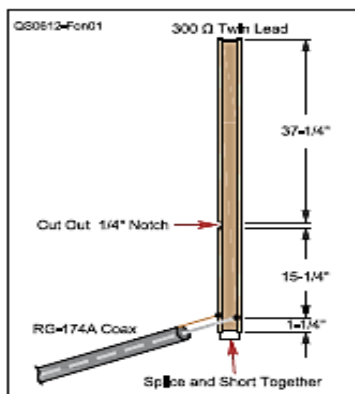
Figure 1 — The original 2 meter ribbon J-pole antenna.
