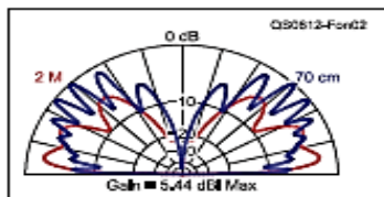
Figure 2 — Elevation plane pattern comparing 2 meter J-pole on fundamental and on third harmonic frequency (70 cm), with the antenna mounted 8 feet above ground. Most of the energy at the third harmonic is launched at 44°.
